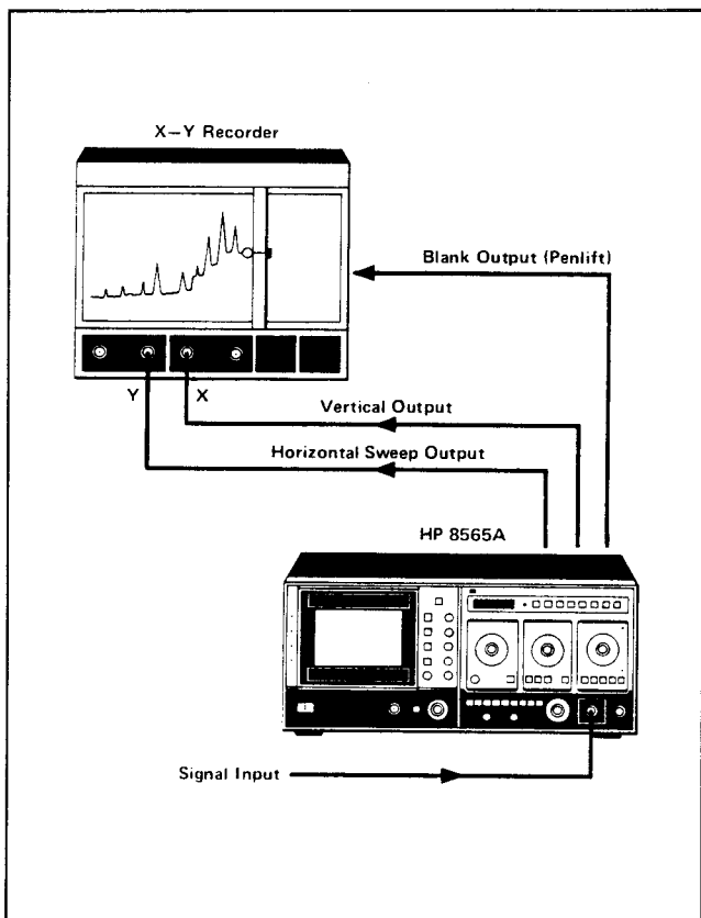
Figure 19. X-Y recording
