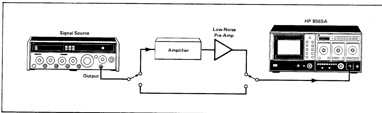
Figure 35. Swept noise figure test set-up
